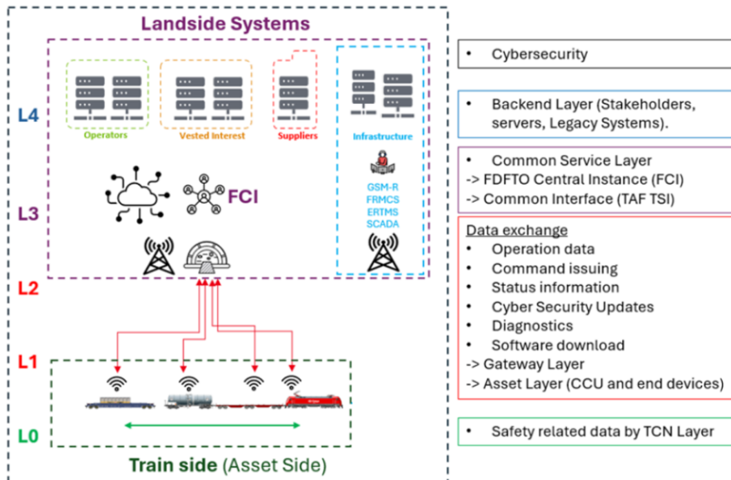
Figure 7 Abstract IT Architecture of the DFOTO system
