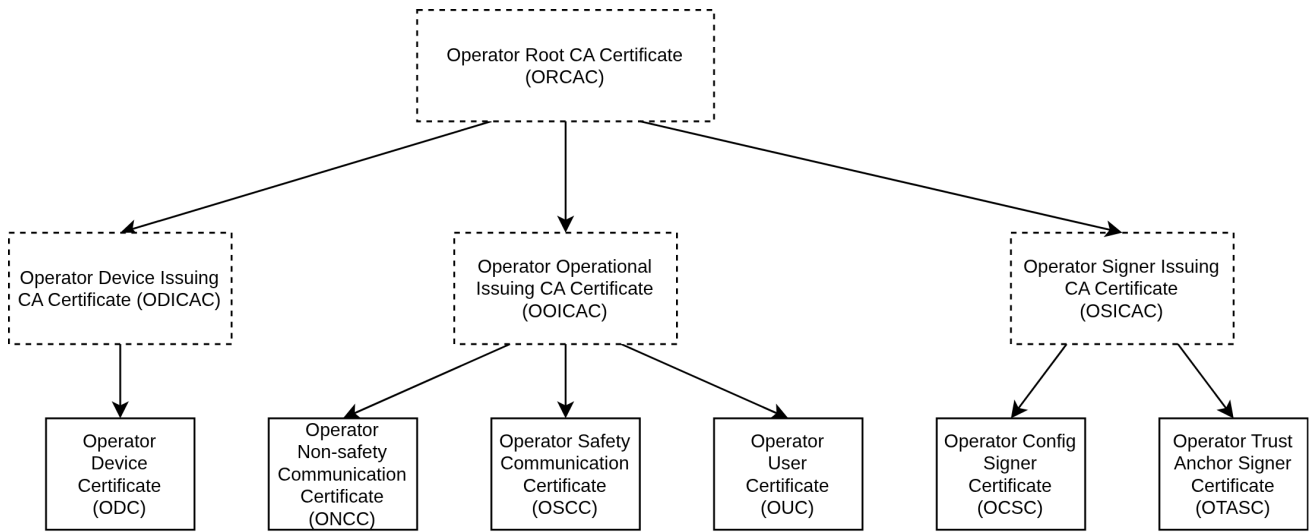
Figure 8 Operator PKI Hierarchy (ECC). Certificates with solid lines are defined by certificate profiles.
