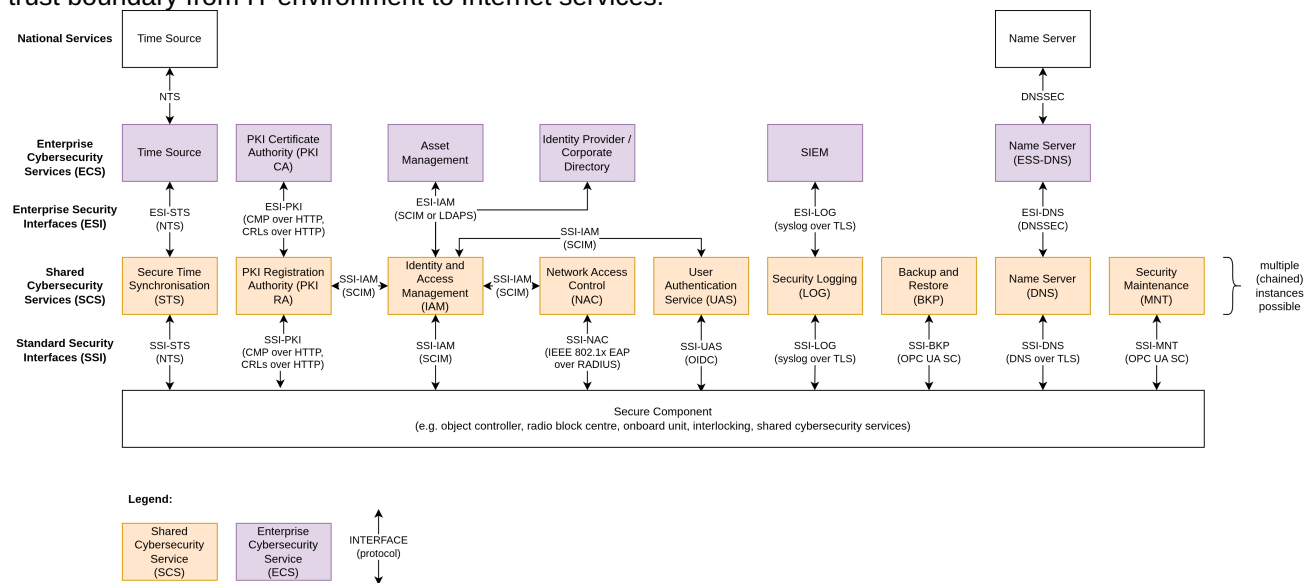
Figure 1 Overview of the Shared Cybersecurity Services and their Interfaces
