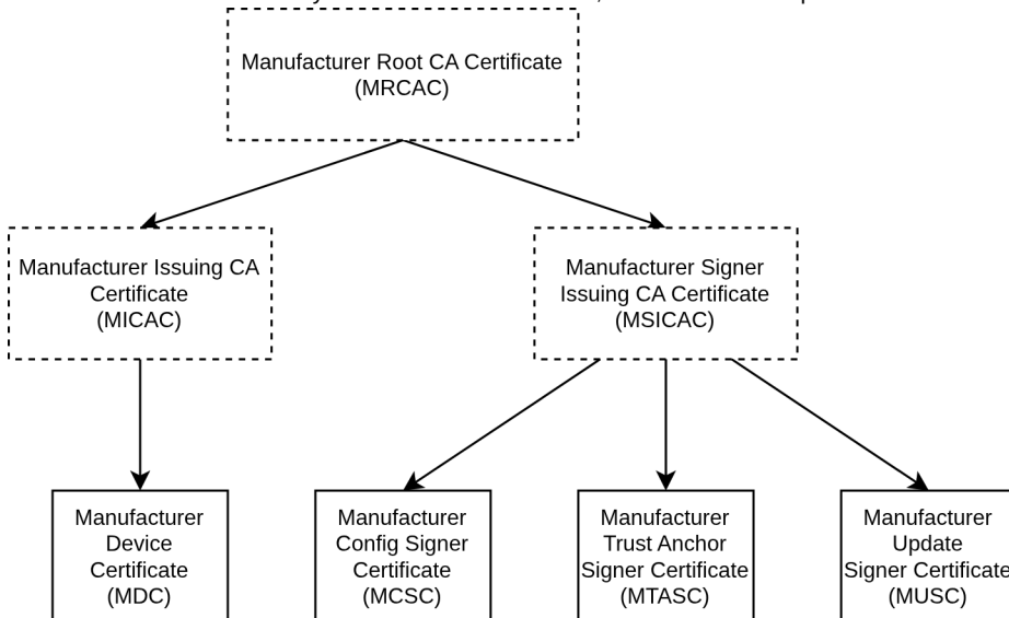
Figure 7 Manufacturer PKI Hierarchy. Certificates with solid lines are defined by certificate profiles. [SPPRAMSS-5650 ]
