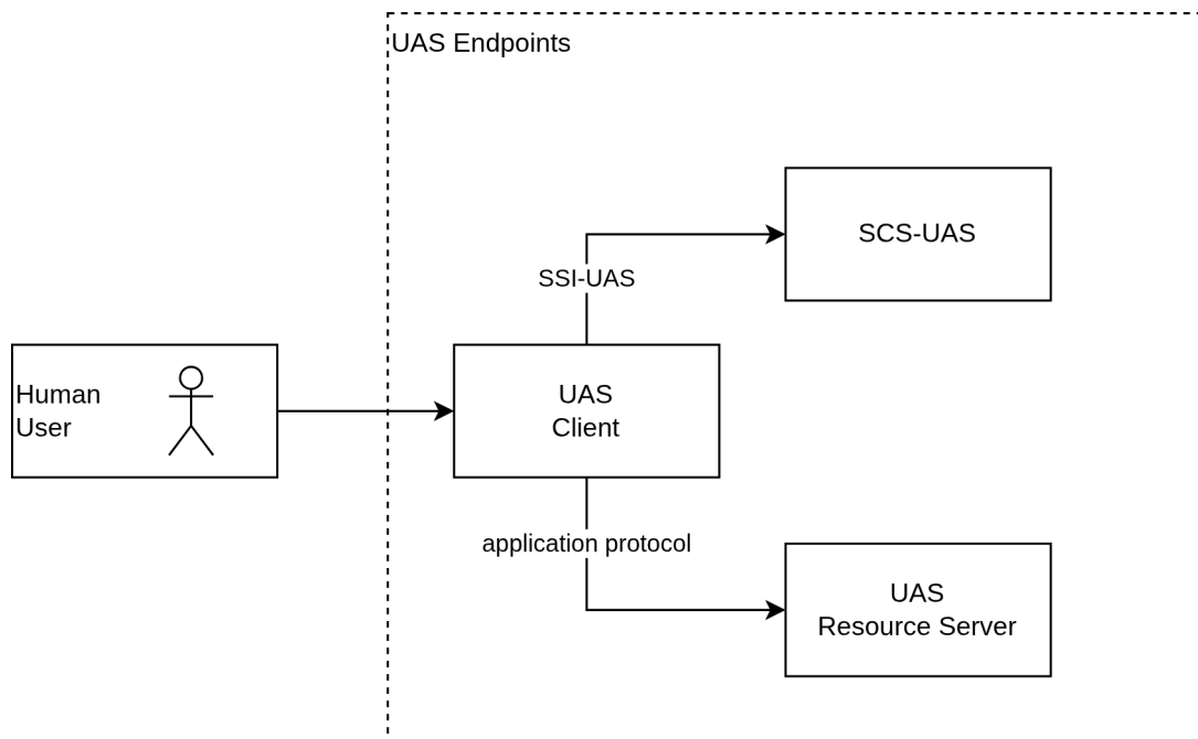
Figure 12 Endpoints of the User Authentication Service (UAS)
