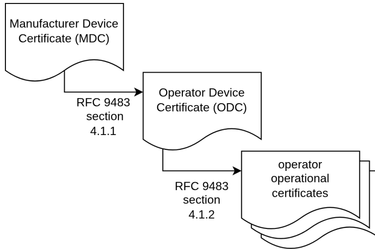
Figure 6 Dependencies of Certificates with References to CMP RFC
