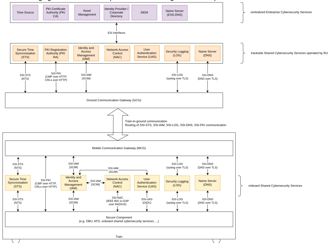
Figure 2 Example architecture of onboard and trackside Shared Cybersecurity Services
