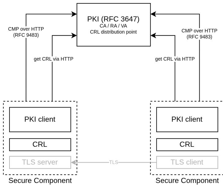
Figure 5 Interface between PKI and Secure Components
