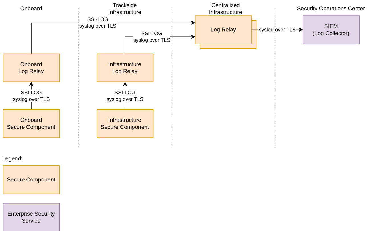
Figure 11 Exemplary Architecture of the Log Services
