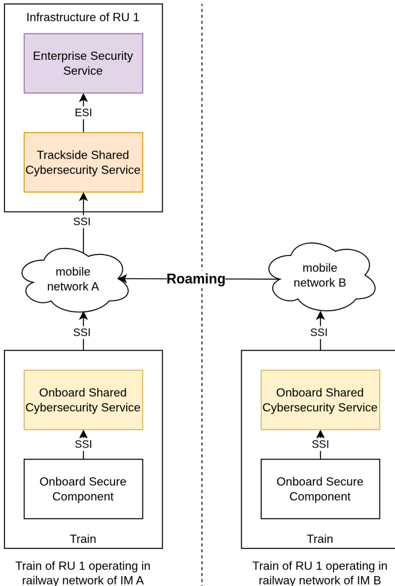
Figure 3 Roaming between networks to reach trackside Shared Cybersecurity Services
