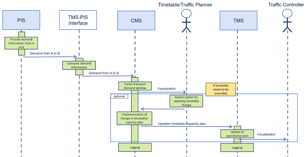
Figure 4: Sequence Diagram SD-WP6-2.2
