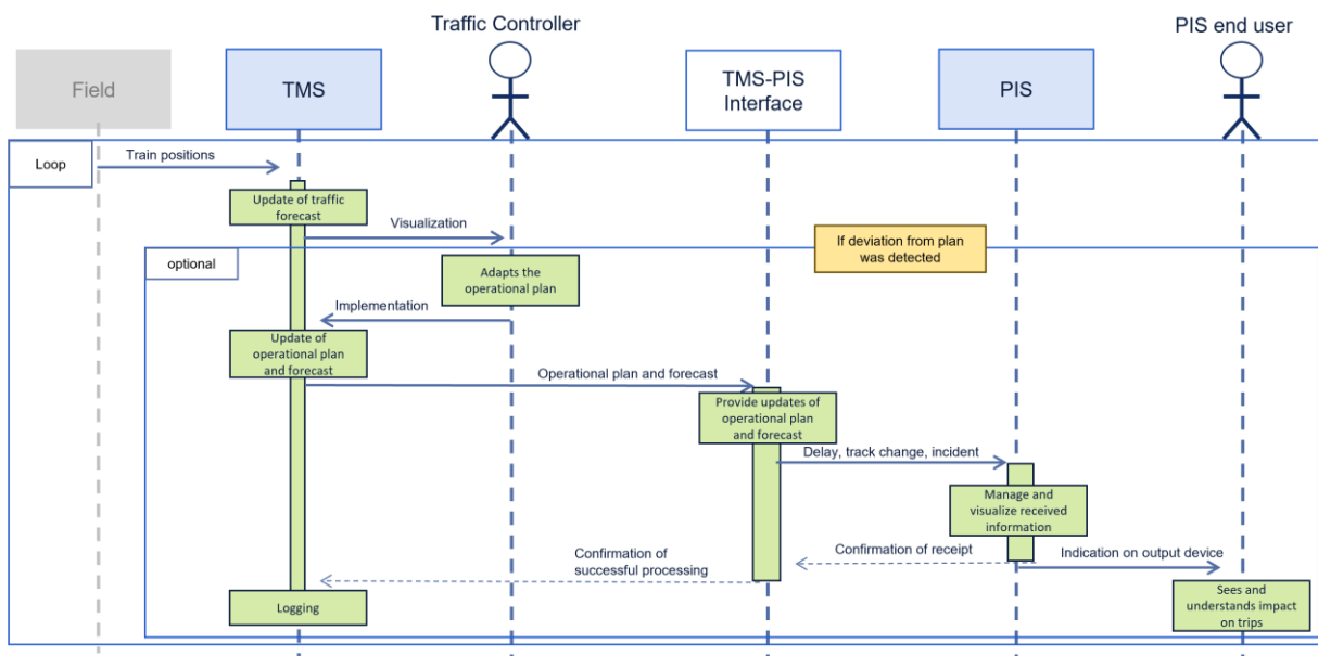
Figure 3: Sequence Diagram SD-WP6-2.1
